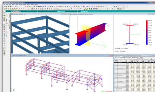
Interactively view stresses on a profile at any cross section on a selected member and load case.
